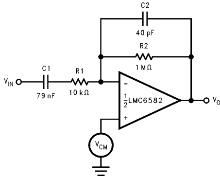
FIGURE 21. Wide-Band Band-Pass Filter
