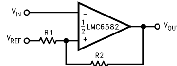
FIGURE 20. Comparator with Hysteresis
