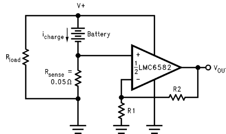
FIGURE 23a. Circuit Used to Sense Charging.
