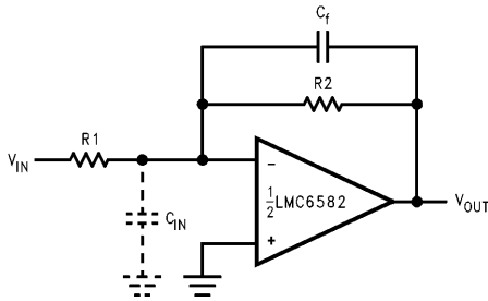
FIGURE 14. Canceling the Effect of Input Capacitance
