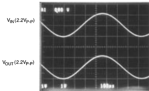
FIGURE 4. The Input Common-Mode Voltage Range Extends to Both Supplies at V_S = 2.2V
