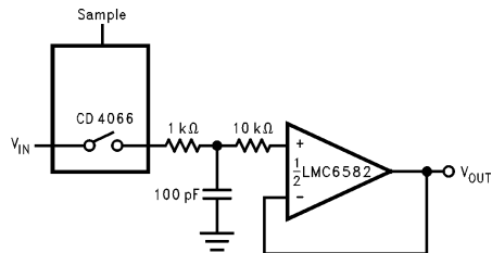
FIGURE 22. Sample-and-Hold Application
