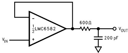
FIGURE 7. Resistive Isolation of a 350 pF Capacitive Load
