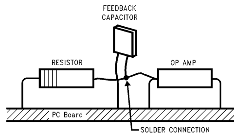
FIGURE 13. Air Wiring
