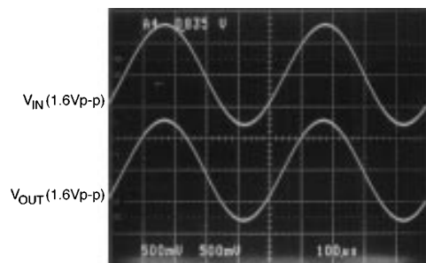
FIGURE 5. Response of the LMC6582/4 at V_S = 1.8V
