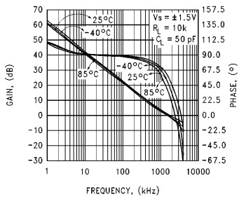
Frequency Response vs Temperature
