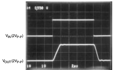
FIGURE 8. Pulse Response of the LMC6582 Circuit in Figure 7
