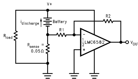
FIGURE 23b. Circuit used to Sense Discharging
