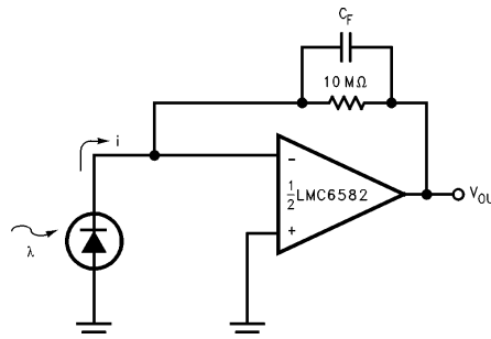
FIGURE 17. Photodiode Amplifier
