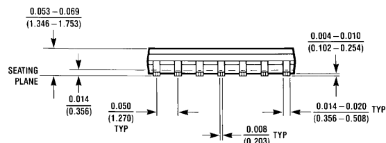
14-Pin Small Outline Package Order Number LMC6584AIM or LMC6584BIM NS Package Number M14A
