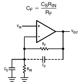
FIGURE 2. General Operational Amplifier Circuit
