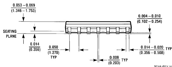
Small Outline Dual-In-Line Pkg. (M) Order Number LMC660AIM, LMC660CM or LMC660EM NS Package Number M14A
