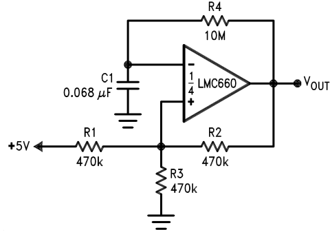
1 Hz Square-Wave Oscillator
