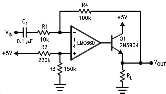
Power Amplifier
