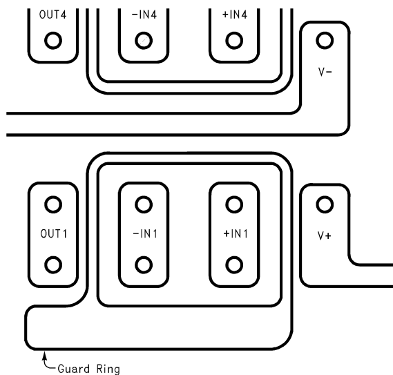
FIGURE 5. Example, using the LMC660AIMEP, of Guard Ring in P.C. Board Layout
