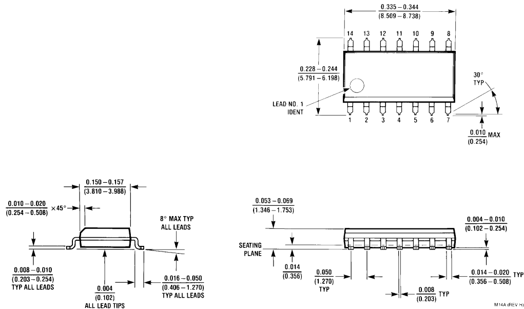
Small Outline Dual-In-Line Pkg. (M) Order Number LMC660AIM, LMC660CM or LMC660EM NS Package Number M14A
