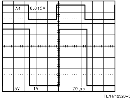
FIGURE 1. An Input Signal Exceeds the LMC6762 Power Supply Voltages with No Output Phase Inversion
