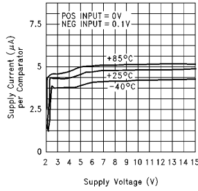
Supply Current vs Supply Voltage (Output Low)
