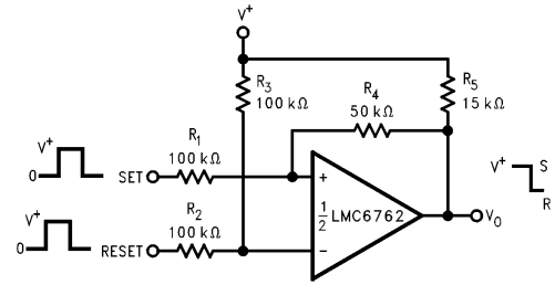
FIGURE 7. Bi-Stable Multivibrator
