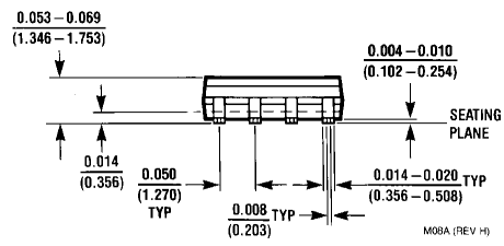
8-Pin Small Outline Package Order Number LMC6762AI or LMC6762BI NS Package Number M08A
