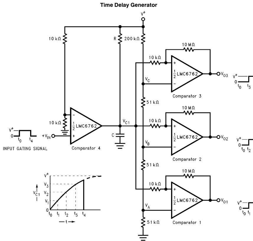
FIGURE 10. Time Delay Generator
