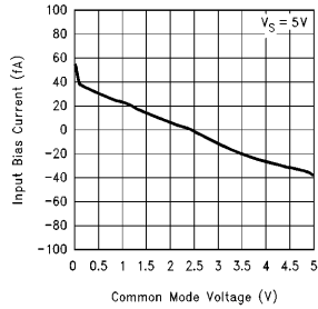
Input Current vs Common-Mode Voltage
