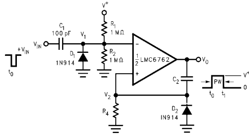
FIGURE 6. One-Shot Multivibrator
