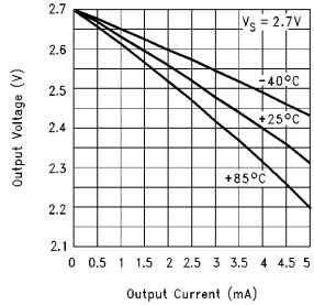
Output Voltage vs Output Current (Sourcing)
