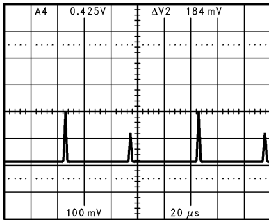
FIGURE 4. Measurement of the Shoot-Through Current
