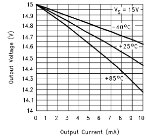
Output Voltage vs Output Current (Sourcing)
