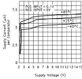
Supply Current vs Supply Voltage (Output High)
