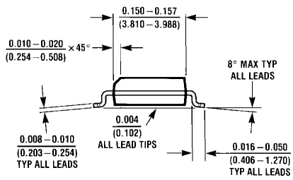
8-Pin Small Outline Package Order Number LMC6762AI or LMC6762BI NS Package Number M08A
