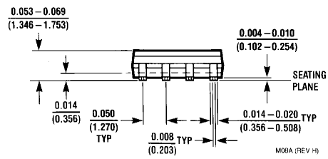
8-Pin Small Outline Package Order Number LMC6772AI or LMC6772BI NS Package Number M08A
