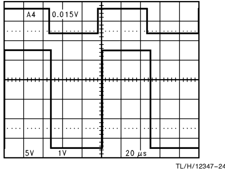
FIGURE 1. An Input Signal Exceeds the LMC6772 Power Supply Voltages with No Output Phase Inversion
