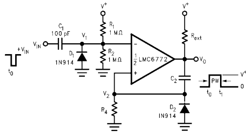
FIGURE 5. One-Shot Multivibrator
