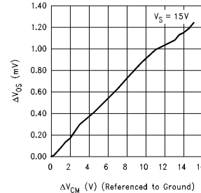
\Delta V_{OS} vs \Delta V_{CM} V_S = 15V
