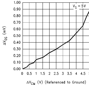
\Delta V_{OS} vs \Delta V_{CM} V_S = 5V
