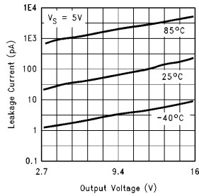
Leakage Current vs Output Voltage
