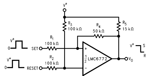
FIGURE 6. Bi-Stable Multivibrator
