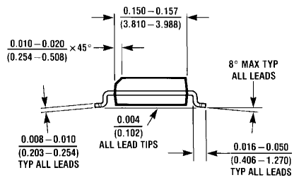
8-Pin Small Outline Package Order Number LMC6772AI or LMC6772BI NS Package Number M08A
