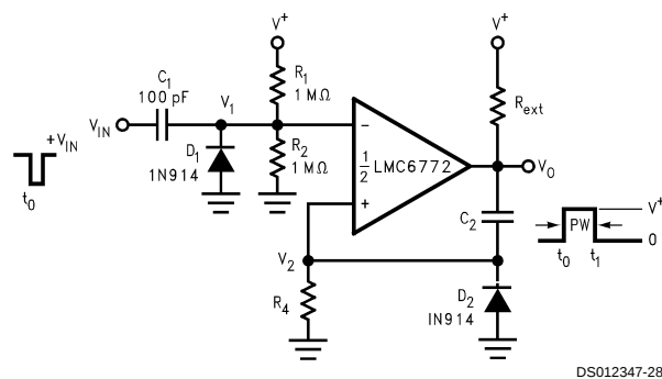
FIGURE 5. One-Shot Multivibrator
