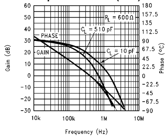
Gain and Phase vs Capacitance Load (2.7V)
