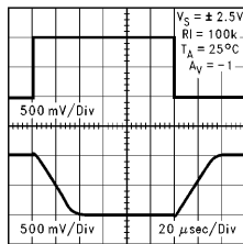
Inverting Large Signal Pulse Response at 5V
