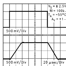
Non-Inverting Large Signal Pulse Response at 5V
