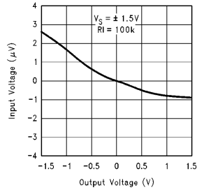
Output Voltage vs Input Voltage @ 3V
