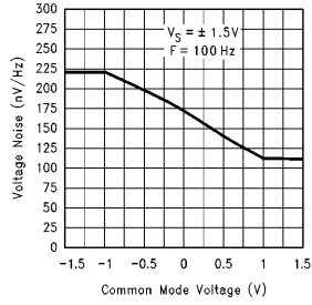
Voltage Noise vs Common Mode Voltage @ 3V
