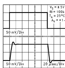
Non-Inverting Small Signal Pulse Response at 10V
