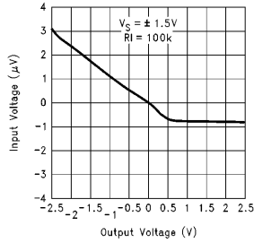
Output Voltage vs Input Voltage @ 5V
