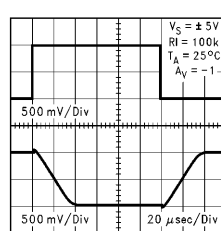
Inverting Large Signal Pulse Response at 10V
