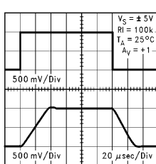
Non-Inverting Large Signal Pulse Response at 10V
