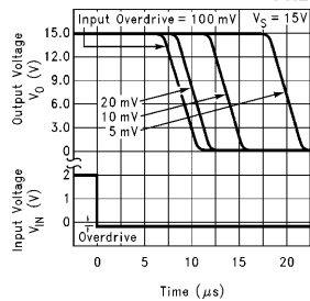
Response Time for Various Input Overdrives — t_{PHL}
