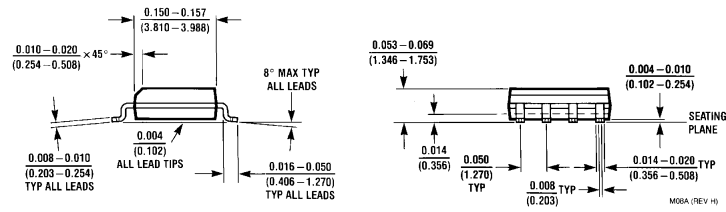
8-Pin Small Outline Package Order Number LMC7211AIM or LMC7211BIM NS Package Number M08A
