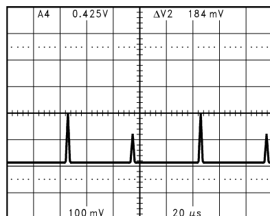
FIGURE 3. Measurement of the Shoot-Through Current
