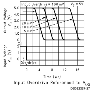
Response Time for Various Input Overdrives -t_{PHL}
