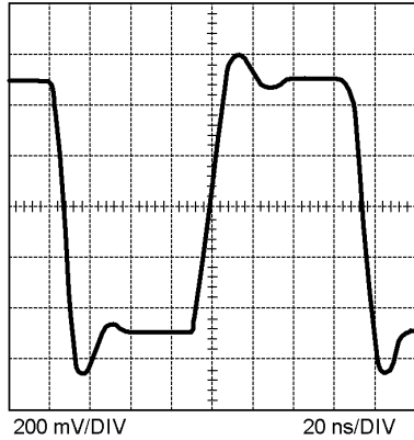
FIGURE 4. Converter Step Response (1V PP , 20 ns/DIV)
