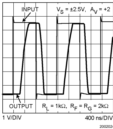
Output Overload Recovery
