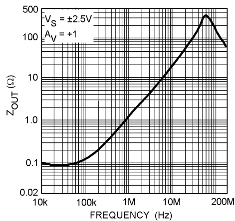
Z_{OUT} vs. Frequency
