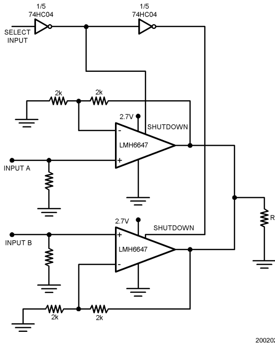
FIGURE 5. 2:1 MUX Operating off a 2.7V Single Supply
