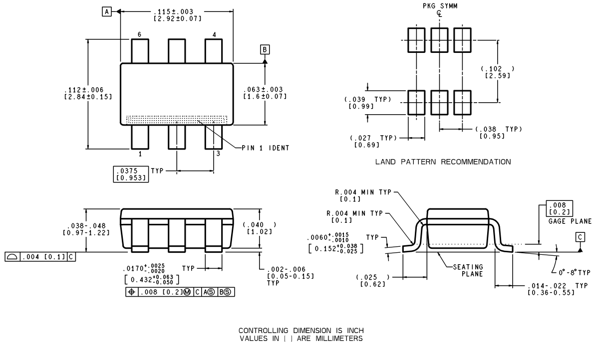
6-Pin SOT23 NS Package Number MF06A
