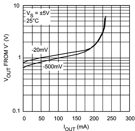
FIGURE 5. I_{SINK} vs. V_{OUT} (for Various Overdrive)
