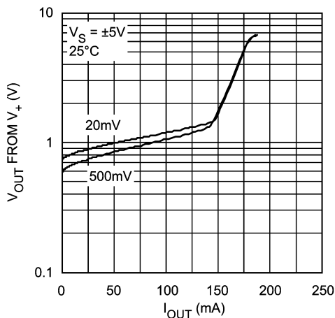
FIGURE 4. I_{SOURCE} vs. V_{OUT} (for Various Overdrive)
