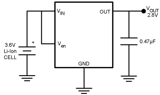
FIGURE 2. Single-Cell Regulator
