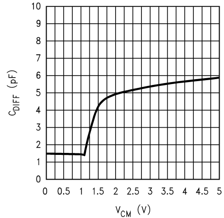
C_{DIFF} vs. V_{CM} ( V_S = 5V )
