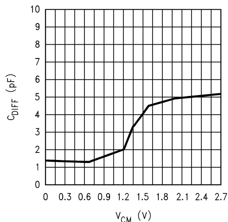
C_{DIFF} vs. V_{CM} ( V_S = 2.7V )
