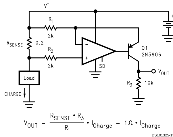
FIGURE 8. High Side Current Sensing
