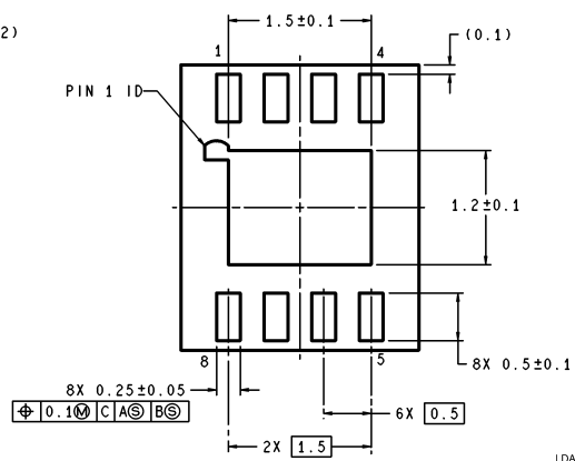
8-Pin LLP NS Package Number LDA08C
