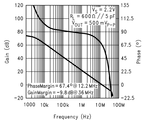
Gain and Phase Margin vs. Frequency ( V_S = 2.2\text{V} , R_L = 600\Omega )
