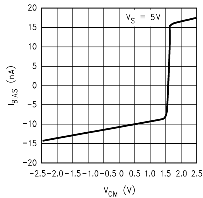
Input Bias Current vs. V_{\text{CM}}
