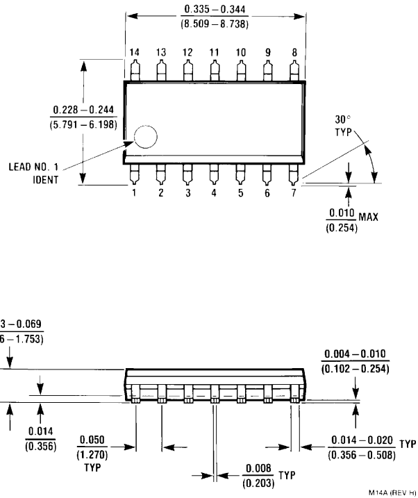
14-Pin SOIC NS Package Number MA14
