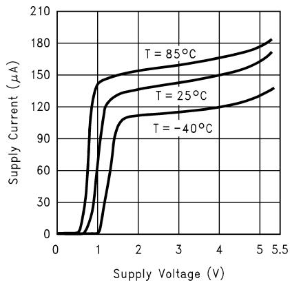
Supply Current vs. Supply Voltage (LMV921)
