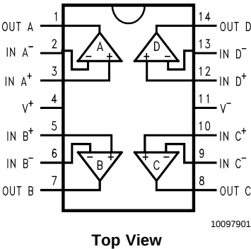
14-Pin TSSOP/SOIC
