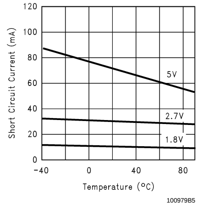
Short Circuit Current vs. Temperature (sinking)
