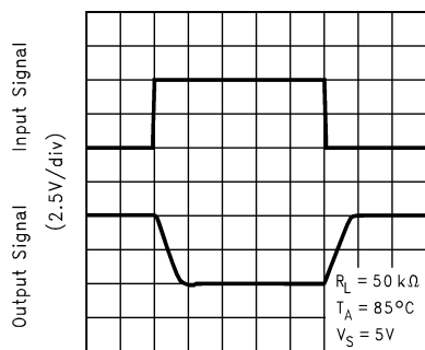
*Large Signal Inverting Response
