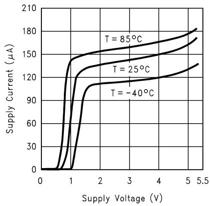
Supply Current vs. Supply Voltage (LMV921)
