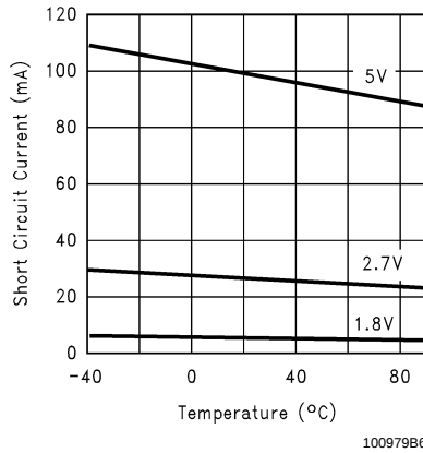
Short Circuit Current vs. Temperature (sourcing)
