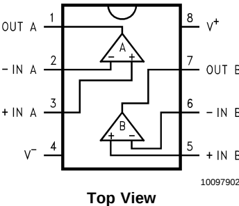
8-Pin MSOP/SOIC
