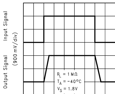
*Large Signal Non-Inverting Response
