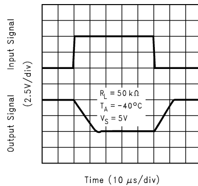
*Large Signal Inverting Response
