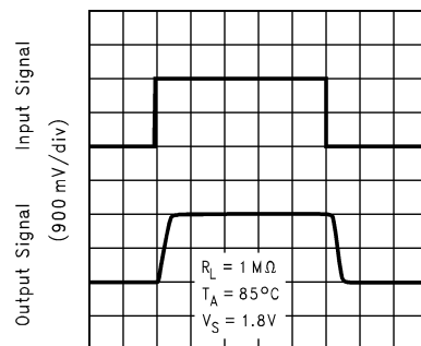
*Large Signal Inverting Response
