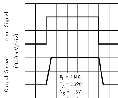
*Large Signal Non-Inverting Response
