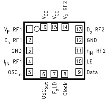
LMX2335U Chip Scale Package (SLB) (Top View)
