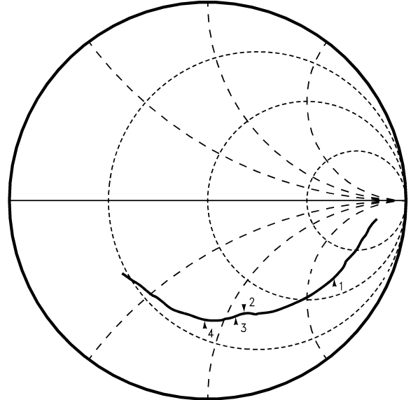
LMX2335U TSSOP and LMX2336U TSSOP f_{IN} RF1 and f_{IN} RF2 Input Impedance V_{CC} = 5.5V, T_A = +25^\circ C
