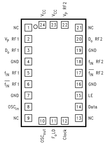
LMX2336U Chip Scale Package (SLB) (Top View)
