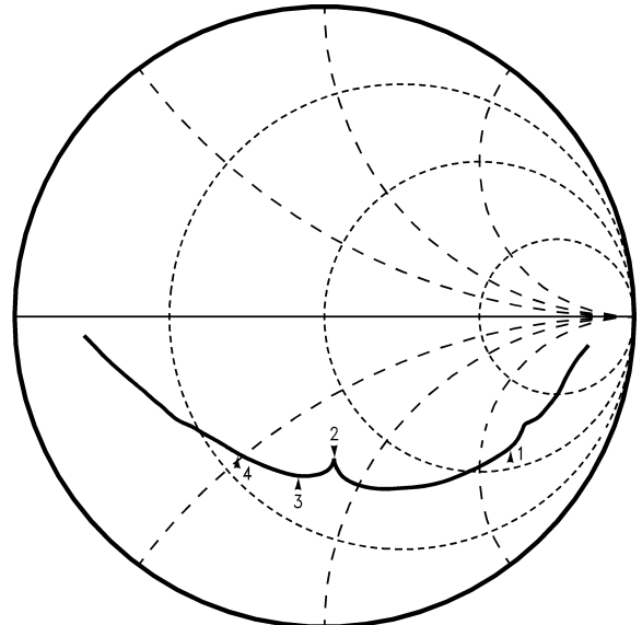
LMX2335U CSP and LMX2336U CSP f_{IN} RF1 and f_{IN} RF2 Input Impedance V_{CC} = 5.5V, T_A = +25^\circ C
