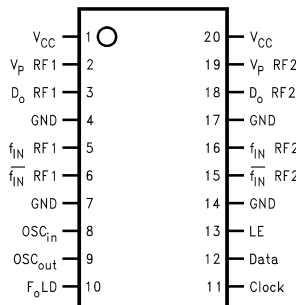
LMX2336U Thin Shrink Small Outline Package (TM) (Top View)
