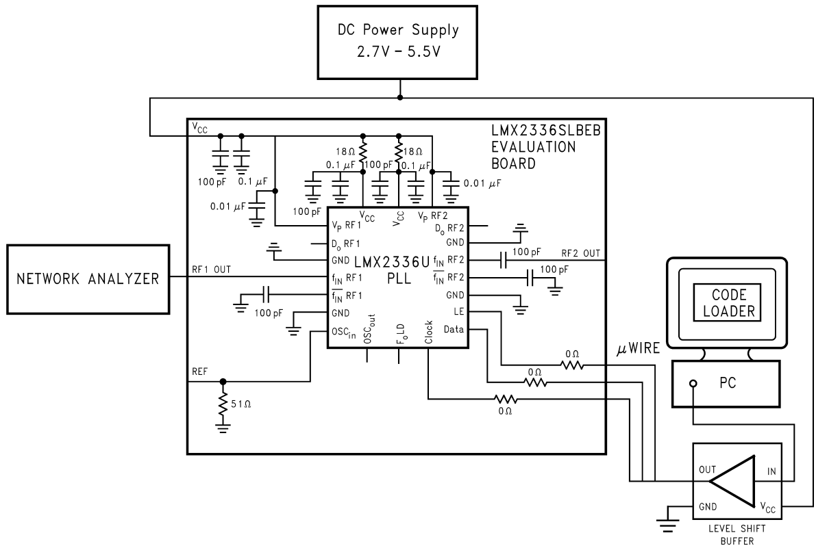
LMX2335U and LMX2336U f_{IN} Impedance Test Setup
