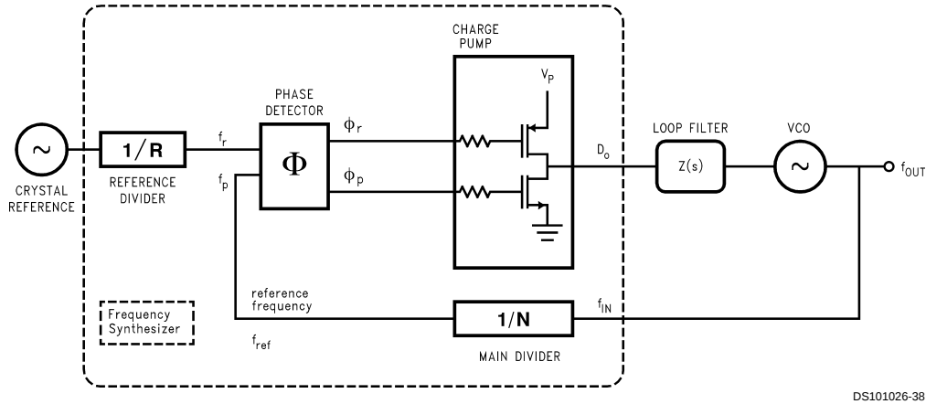
FIGURE 1. Basic Charge Pump Phase Locked Loop
