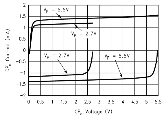
Charge Pump Current vs CP_O Voltage ICP_O = \text{LOW}
