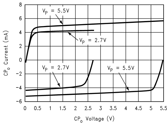
Charge Pump Current vs CP_O Voltage ICP_O = \text{HIGH}
