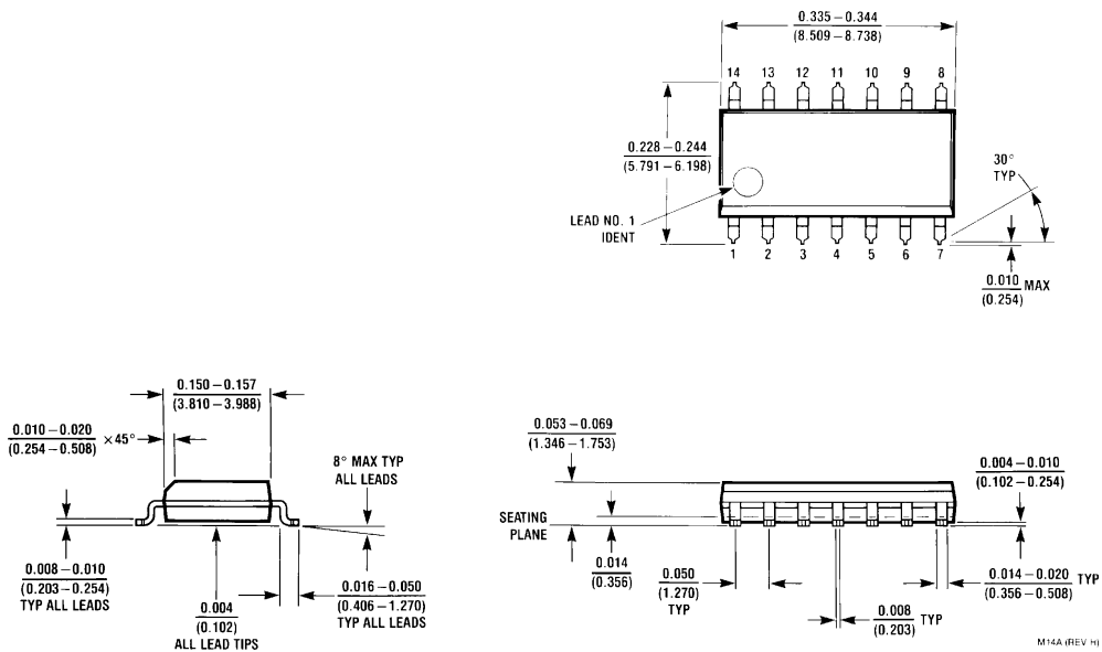
S.O. Package (M) Order Number LP324M or LP2902M NS Package Number M14A
