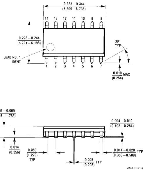
S.O. Package (M) Order Number LP324M or LP2902M NS Package Number M14A
