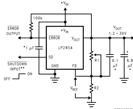
FIGURE 2. Adjustable Regulator
