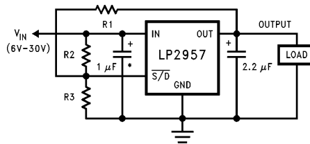
FIGURE 3. Snap-On/Snap-Off Output
