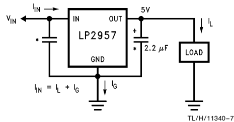
FIGURE 1. Basic 5V Regulator Circuit
