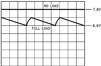
FIGURE 7. V_{IN} VOLTAGE WAVEFORMS
