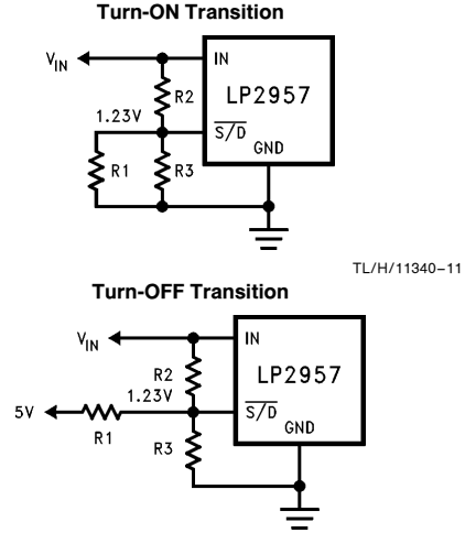
FIGURE 6. Equivalent Circuits
