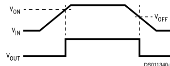
FIGURE 4. Snap-On/Snap-Off Input and Output Voltage Diagram
