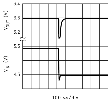
Line Transient Response ( C_{OUT} = 10\mu F , I_{OUT} = 100mA )
