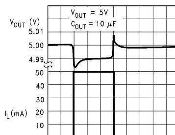
Load Transient Response
