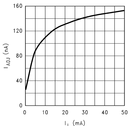
ADJ Pin Bias Current vs. Load Current
