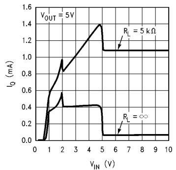
Input Current vs V_{IN}
