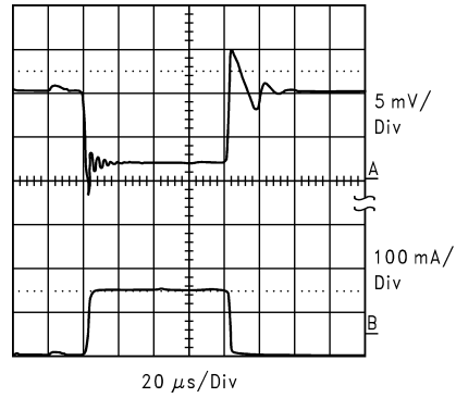
Load Transient Response C_{OUT} = 2.2\mu F
