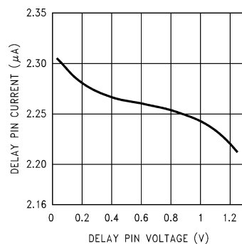
Delay Pin Current vs Delay Pin Voltage
