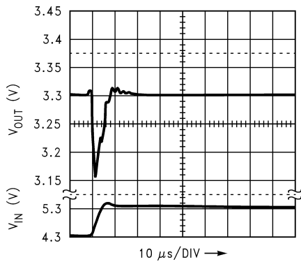
Line Transient Response ( I_{OUT} = 800mA )
