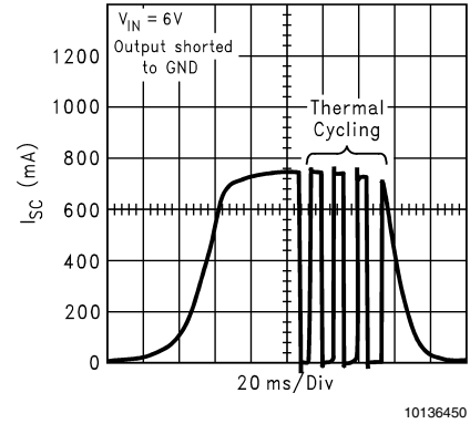
Short Circuit Current ( \mu SMD )
