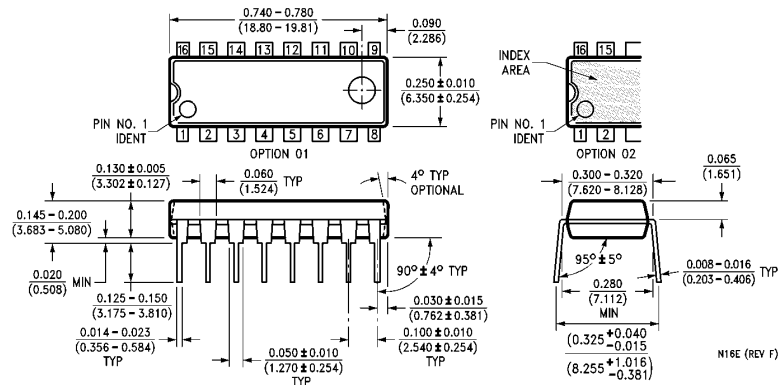
Order Number MM74HC147N NS Package N16E
