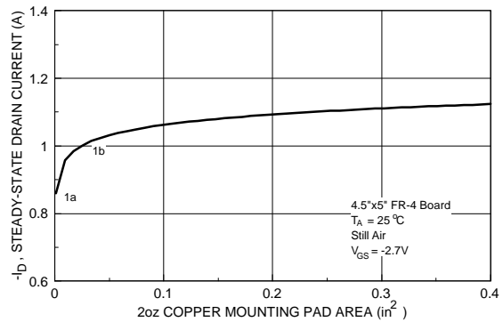
Figure 16. Maximum Steady-State Drain Current versus Copper Mounting Pad.
