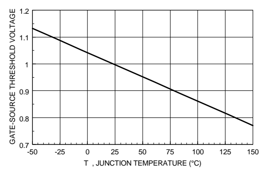
Figure 6. Gate Threshold Variation with Temperature.
