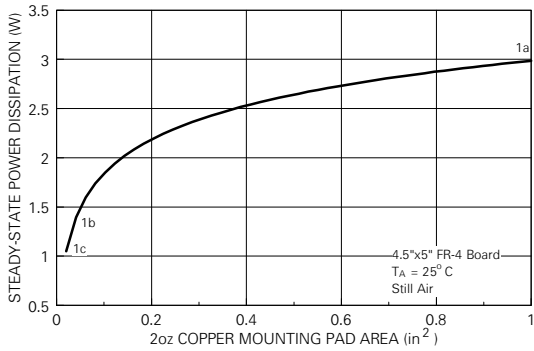
Figure 12. SOT-223 Maximum Steady-State Power Dissipation versus Copper Mounting Pad
