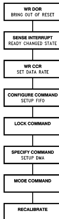
FIGURE 7-2. PC8477B Initialization
