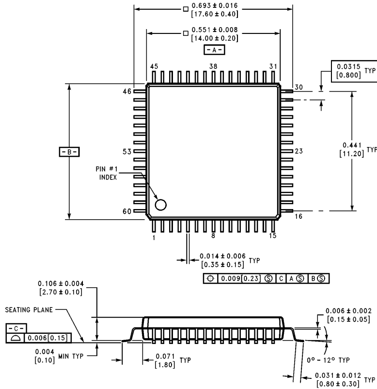
Plastic Quad Flat Package (PQFP) Order Number PC8477BVF-1 NS Package Number VF60A
