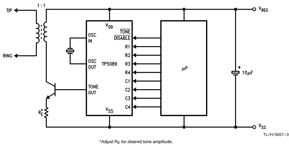
FIGURE 2. Typical Application
