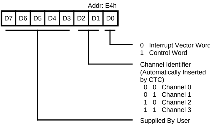
Figure 48. CTC Interrupt Vector Word
