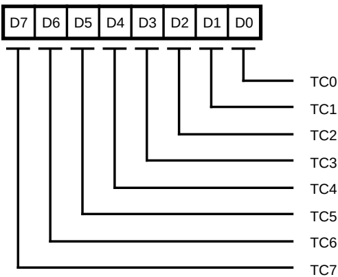
Figure 47. CTC Time Constant Word
