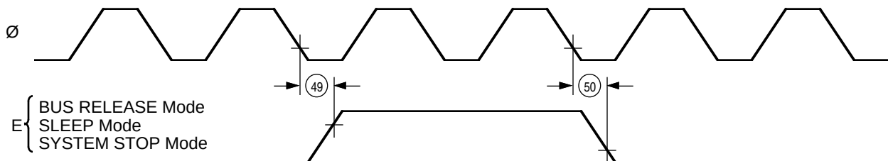
Figure 95. E Clock Timing
