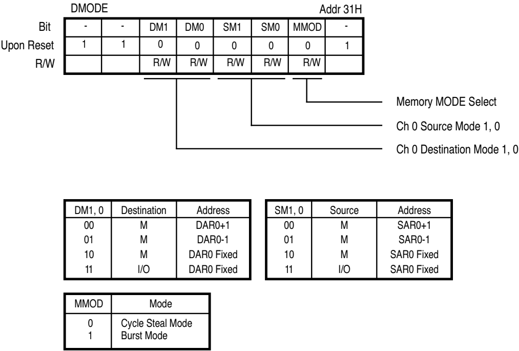
Figure 55. DMA Mode Registers
