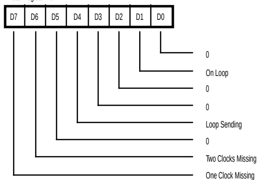
Read Register 10
