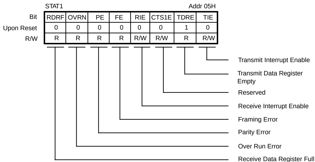
Figure 27. ASCI Status Register (Ch. 1)
