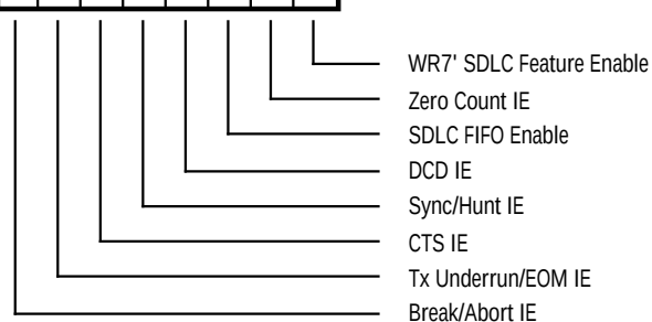
Figure 71. Write Register Bit Functions (Continued)
