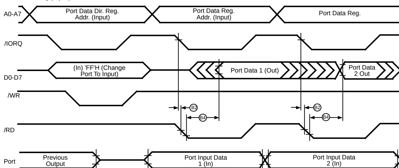
Figure 15. PORT Timing
