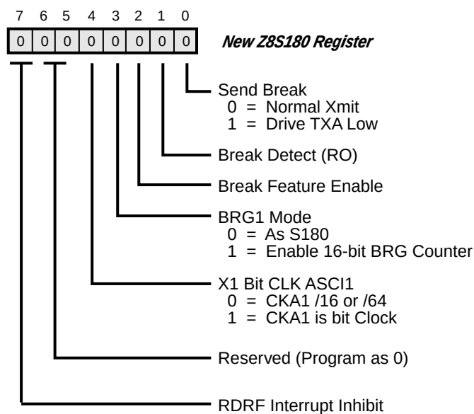
Figure 33. ASCII1 Extension Control Register (I/O Address 13)
