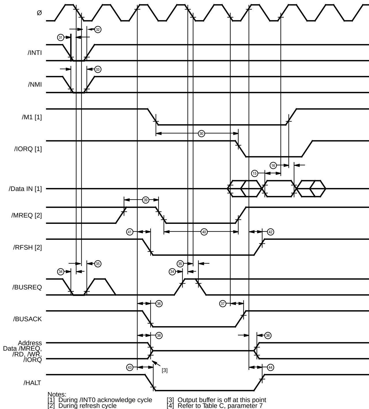
Figure 5. CPU Timing
