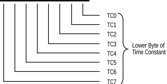
Write Register 12
