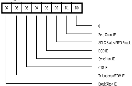
Read Register 15
