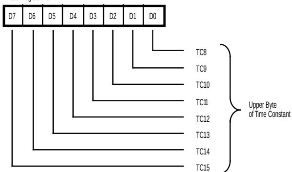
Read Register 13
