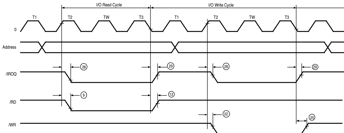
Figure 6. CPU Timing
