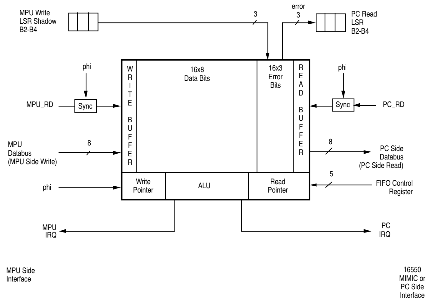
Figure 77. Receiver FIFO Block Diagram
