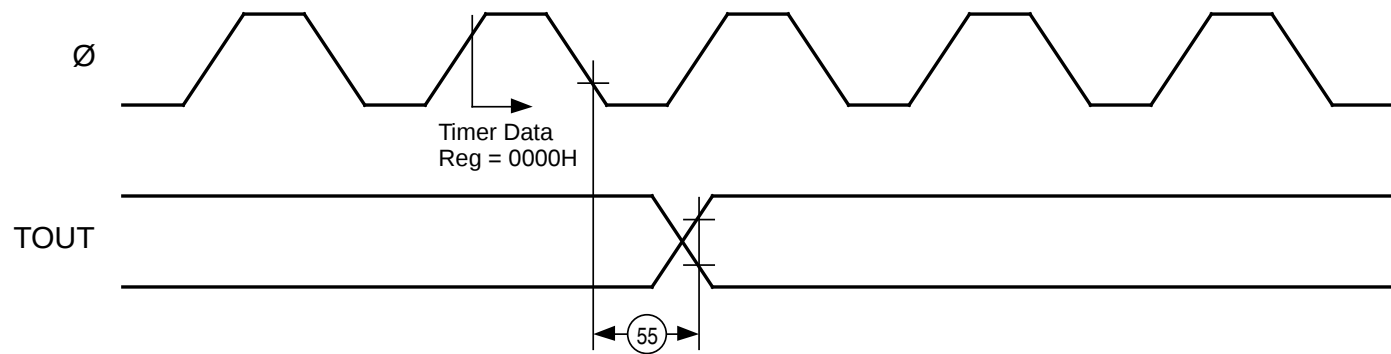
Figure 12. Timer Output Timing
