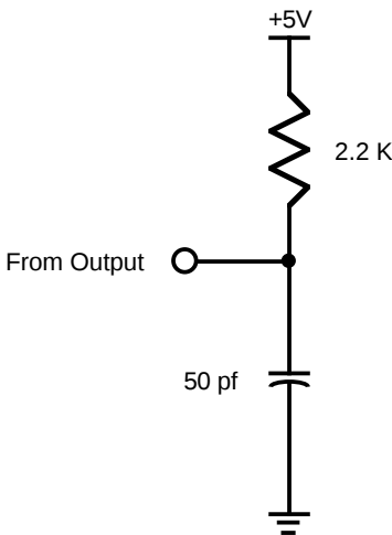
Open-Drain Test Load
