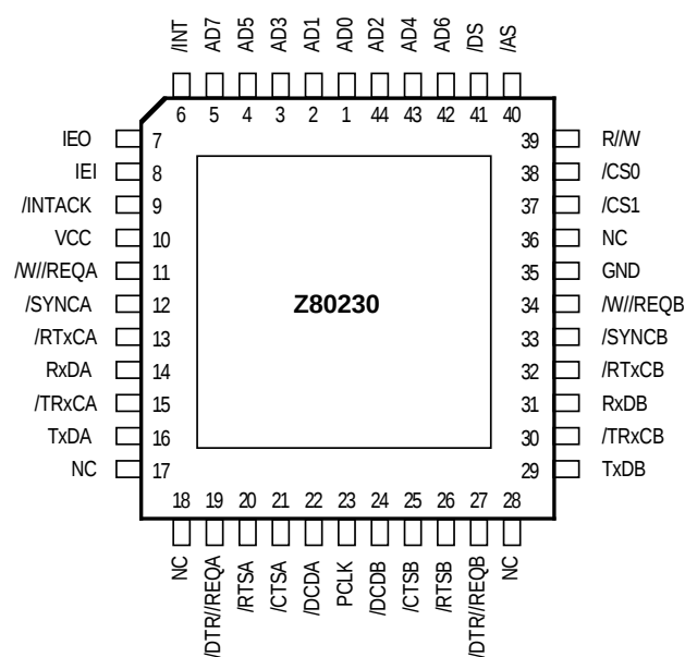
Z80230 PLCC Pin Assignments
