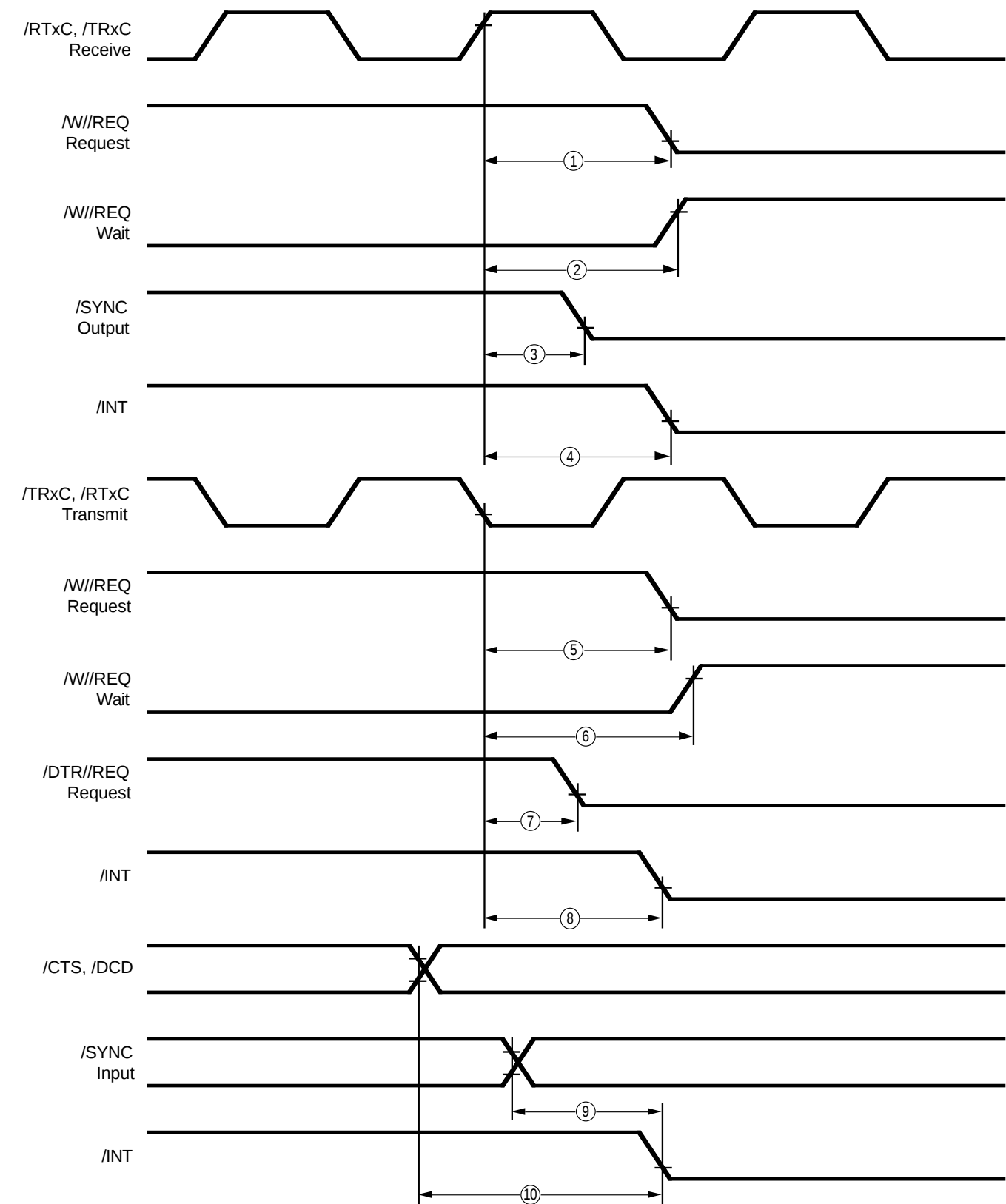
Z80230 System Timing Diagram
