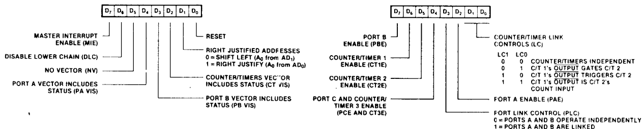
Figure B-1. Master Control Registers
