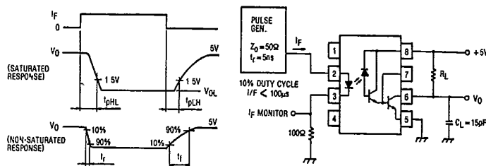
TEST CIRCUIT 1.
